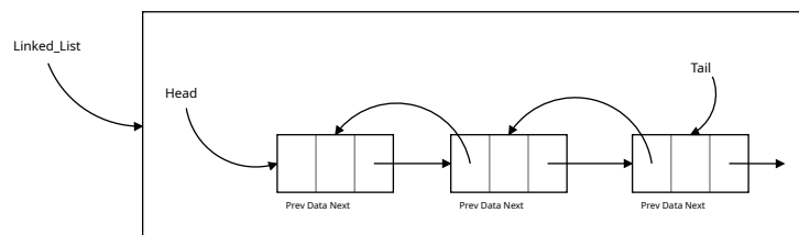
Figure 98: Doubly Linked List Reference Image
